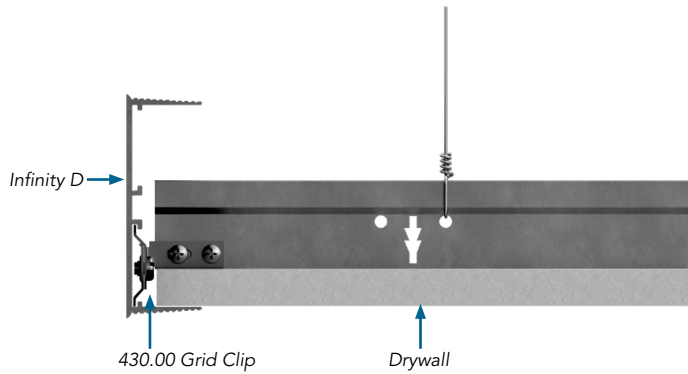
Installation of Infinity with Drywall Grid and Gypsum Board
