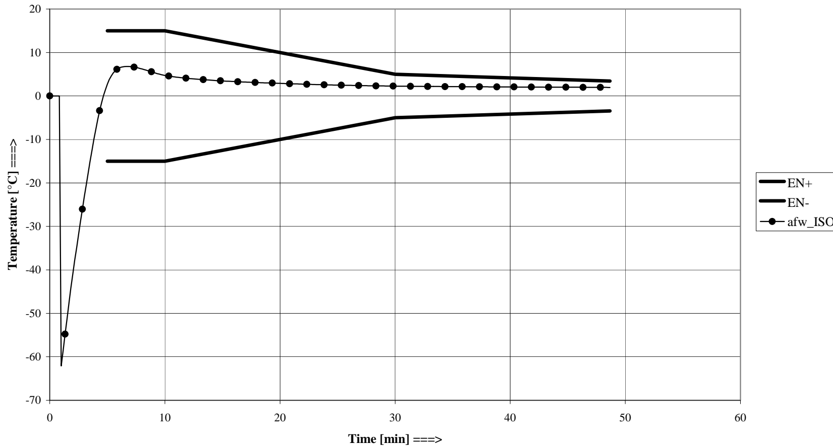
Figure B3: Deviation fire curve
