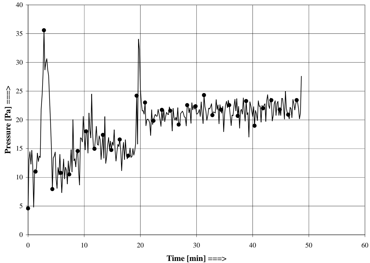
Figure B4: Furnace pressure
