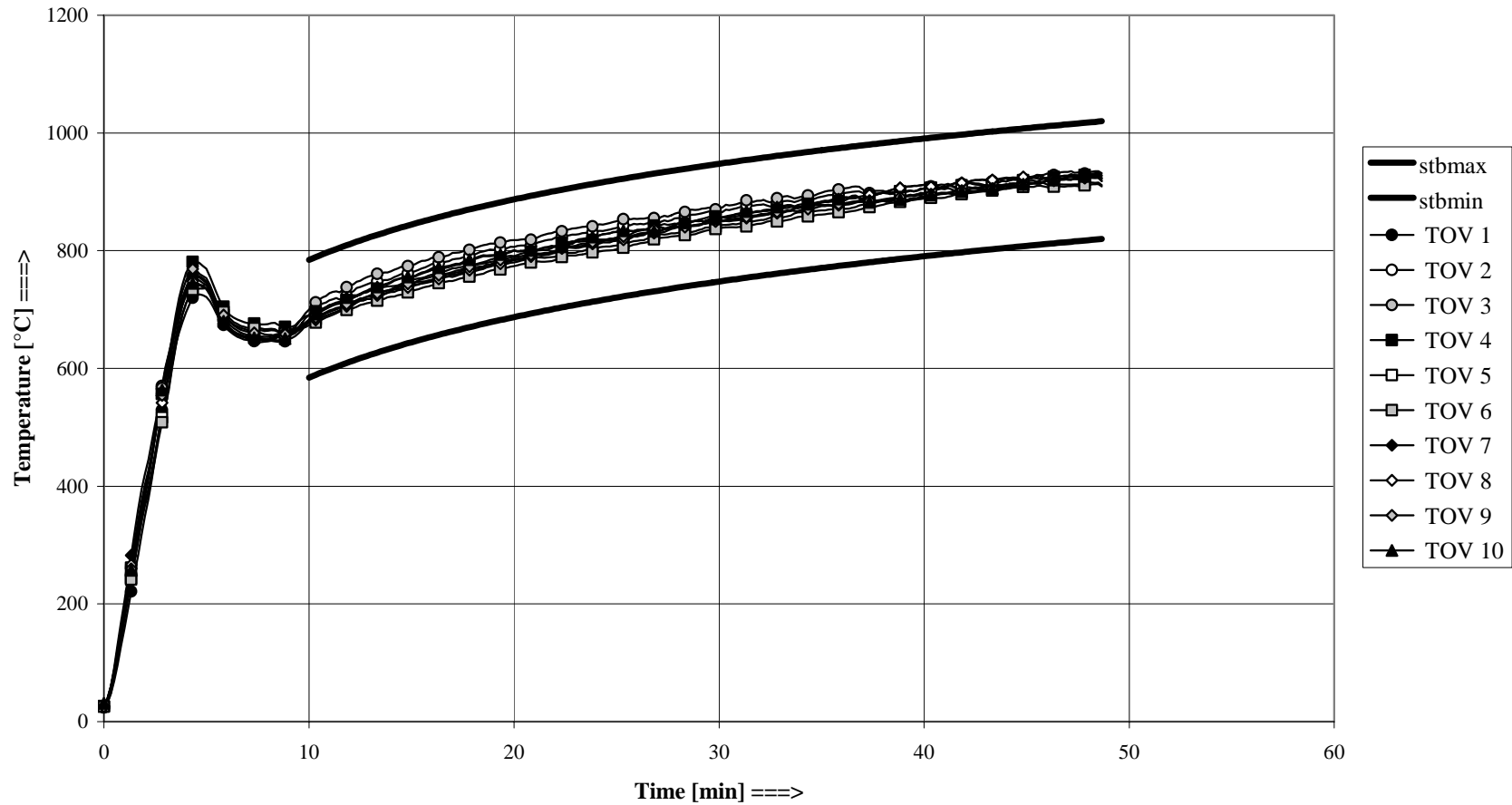
Figure B2: Furnace temperature
