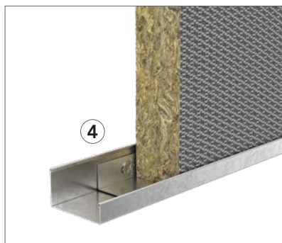
The 40 mm J-channel (25/40/13 mm) and the supporting bracket to support the bottom of the panels mounted at multiple heights or off the floor.
