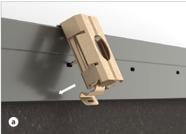
Attach the remaining Mounting Clips using the alignment holes. Hook the Rockfon Lamella Mounting Clips onto the horizontal profiles. Align the pin on the back of the Mounting Clip with the hole on the front face of the horizontal profiles.
