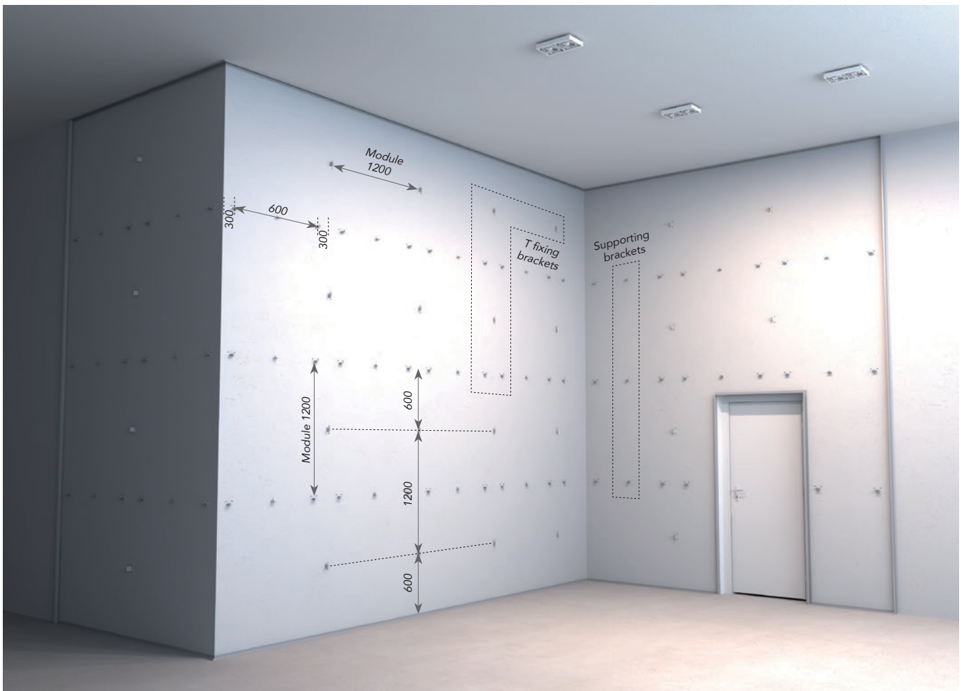
2.1 Placement of all T fixing brackets and supporting brackets should be measured out and mounted before any panel installation begins. Doing so will greatly reduce installation time. Ensure that all brackets line up – T fixing brackets' channel on the module axis, supporting brackets' underside 4 mm above it.
