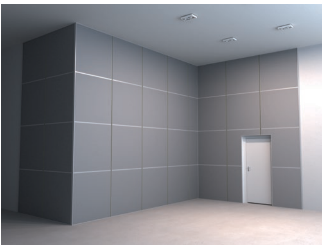
3.11 Install all remaining intermediate panels as described on page 9, working from the top downwards. During installation, cover all horizontal joints with T24 profiles by clicking them into the T fixing brackets. When the entire installation is fitted with Rockfon VertiQ panels, the final step is covering all the vertical joints with long tees clicked into T fixing brackets (see next section).
