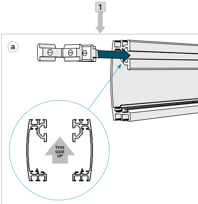
Add the correct amount of Inter Connectors R to the Frame Profiles.
