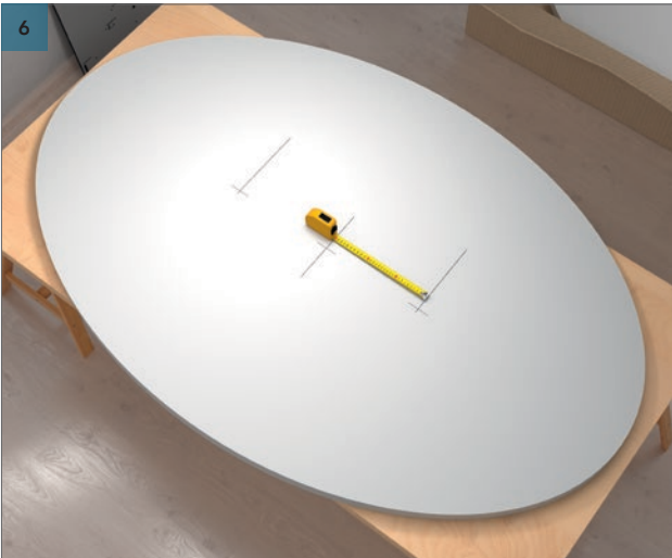
Measure and indicate horizontally 300 mm left and 300 mm right from the center cross.
