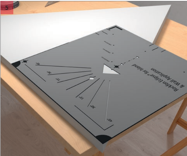
Position the marking tool in the lower corner on the back side of the Eclipse panel, and mark the centre lines using the corner of the marking tool. See 5 - Result.
