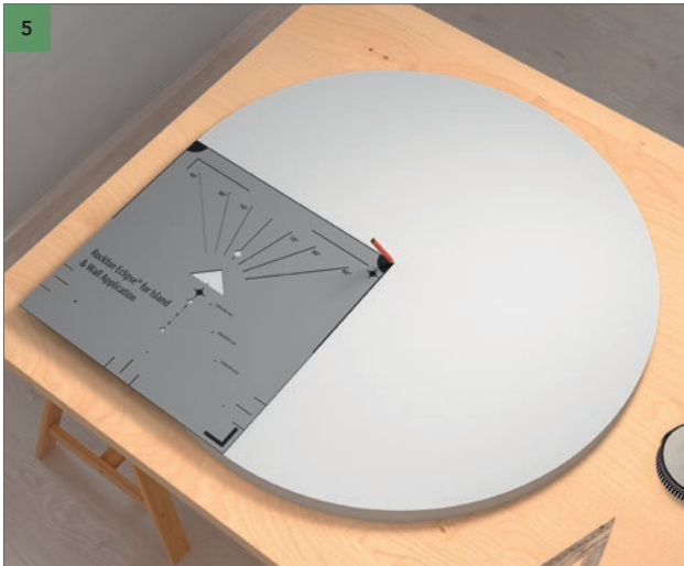
Position the marking tool so the top left and bottom right corners are at the edge of the circle on the back side of the Rockfon Eclipse Wall panel. Mark with a pencil the centre lines using the upper right corner of the marking tool. See 5 - Result.
