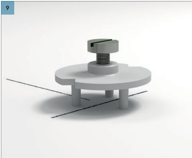
Insert the distance holders (spacer nut M8 with the spacer bolt M8) into the backside of the wall panel. See 9 - Result.
