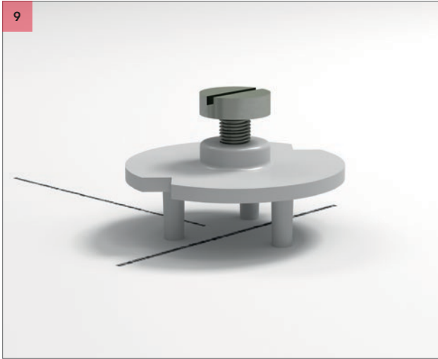
9 Insert the distance holder (spacer nut M8 with the spacer bolt M8) into the backside of the wall panel. See 9 - Result.
