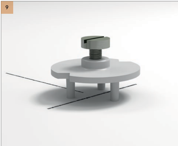
Insert the distance holder (spacer nut M8 with the spacer bolt M8) into the backside of the wall panel. See 9 - Detail.
