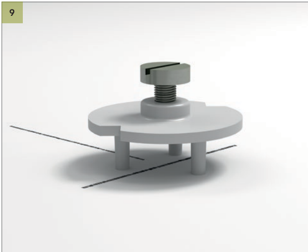
Insert the distance holder (spacer nut M8 with the spacer bolt M8) into the backside of the wall panel. See 9 - Result.
